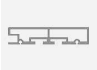
SECTION OF ONLY 20 MM
