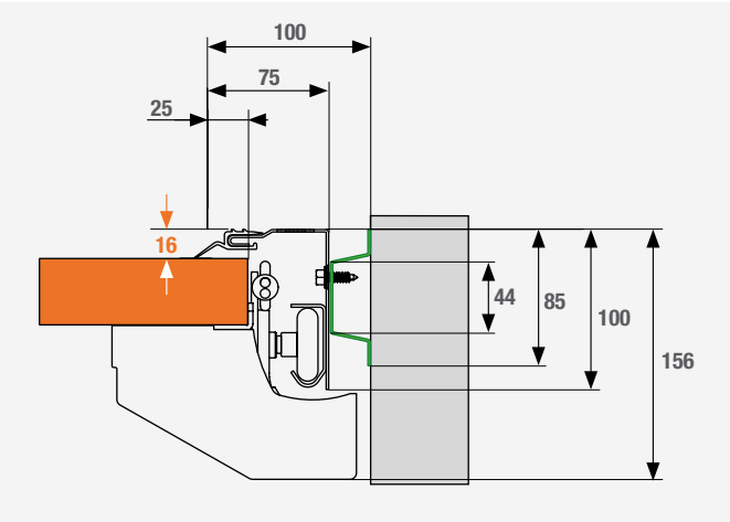
OPTIONAL ASSEMBLY 4 Side mounting with GO-SIDEX system without side space available. Compatible with models GR100NR, GR150NF, GR180NF, GR250NF, GR330NF
