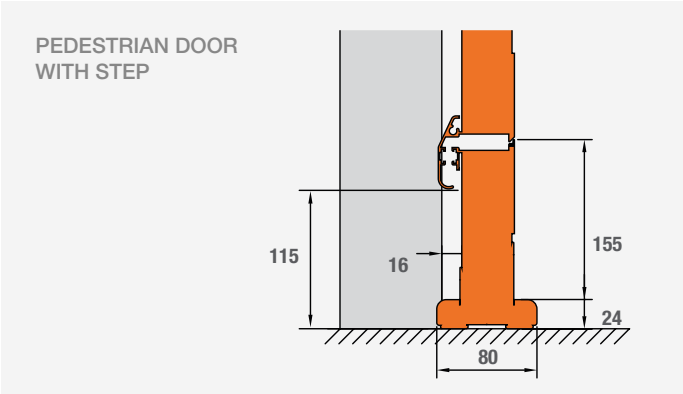
GO-STEP VERTICAL OVERALL SIZES
