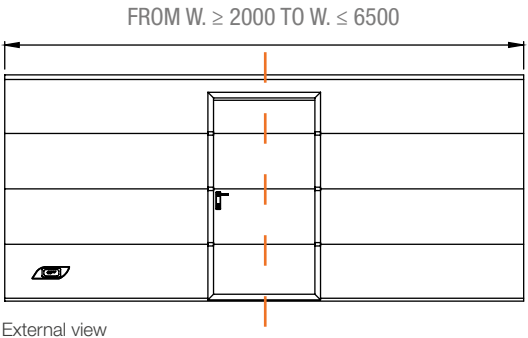
External view
