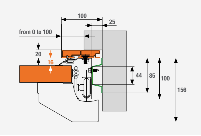
OPTIONAL ASSEMBLY 6 Side mounting with GO-SIDEX system and 100mm side frame GO-XFRAME in partial overlap. Compatible with models GR100NR, GR150NF, GR180NF and GR330NF
