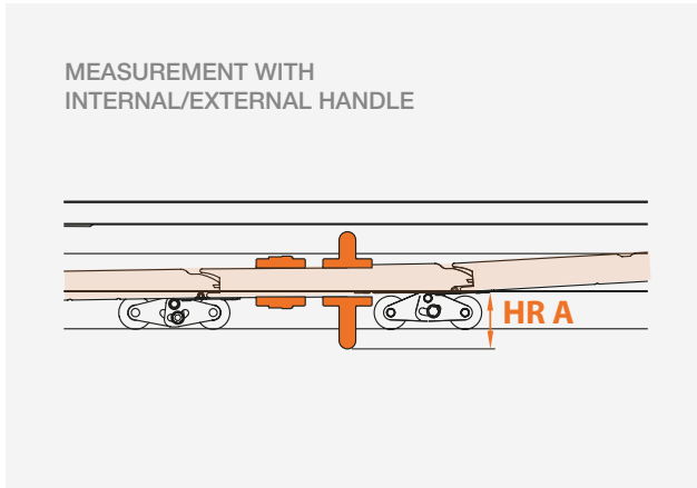
GO-LEVEL / STEP handle measurements with sectional door open
