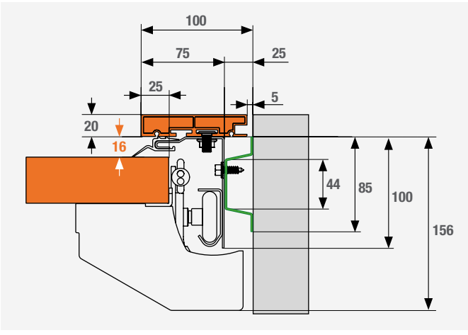
OPTIONAL ASSEMBLY 5 Side mounting with GO-SIDEX system and 100 mm aluminium side frame GO-XFRAME in the opening. Compatible with models GR100NR, GR150NF, GR180NF and GR330NF
