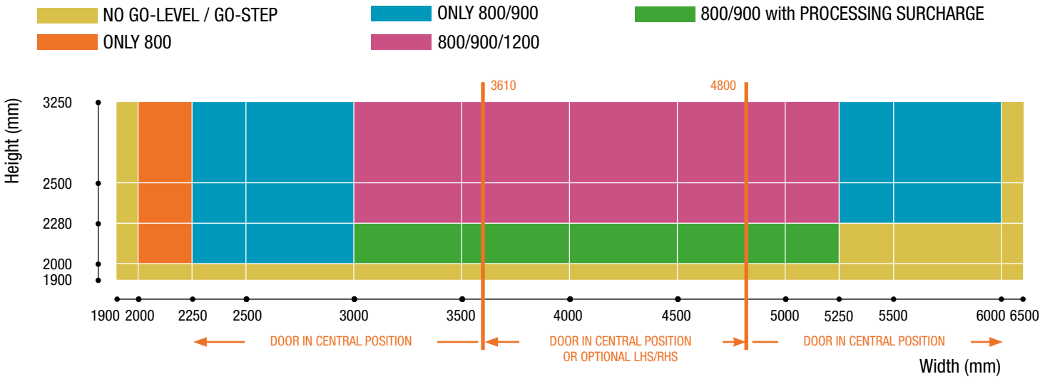
DIAGRAM SHOWING GO-LEVEL / GO-STEP FEASIBILITY ON RESIDENTIAL DOOR
