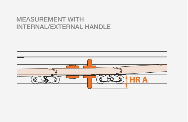
GO-LEVEL / STEP handle measurements with sectional door open
