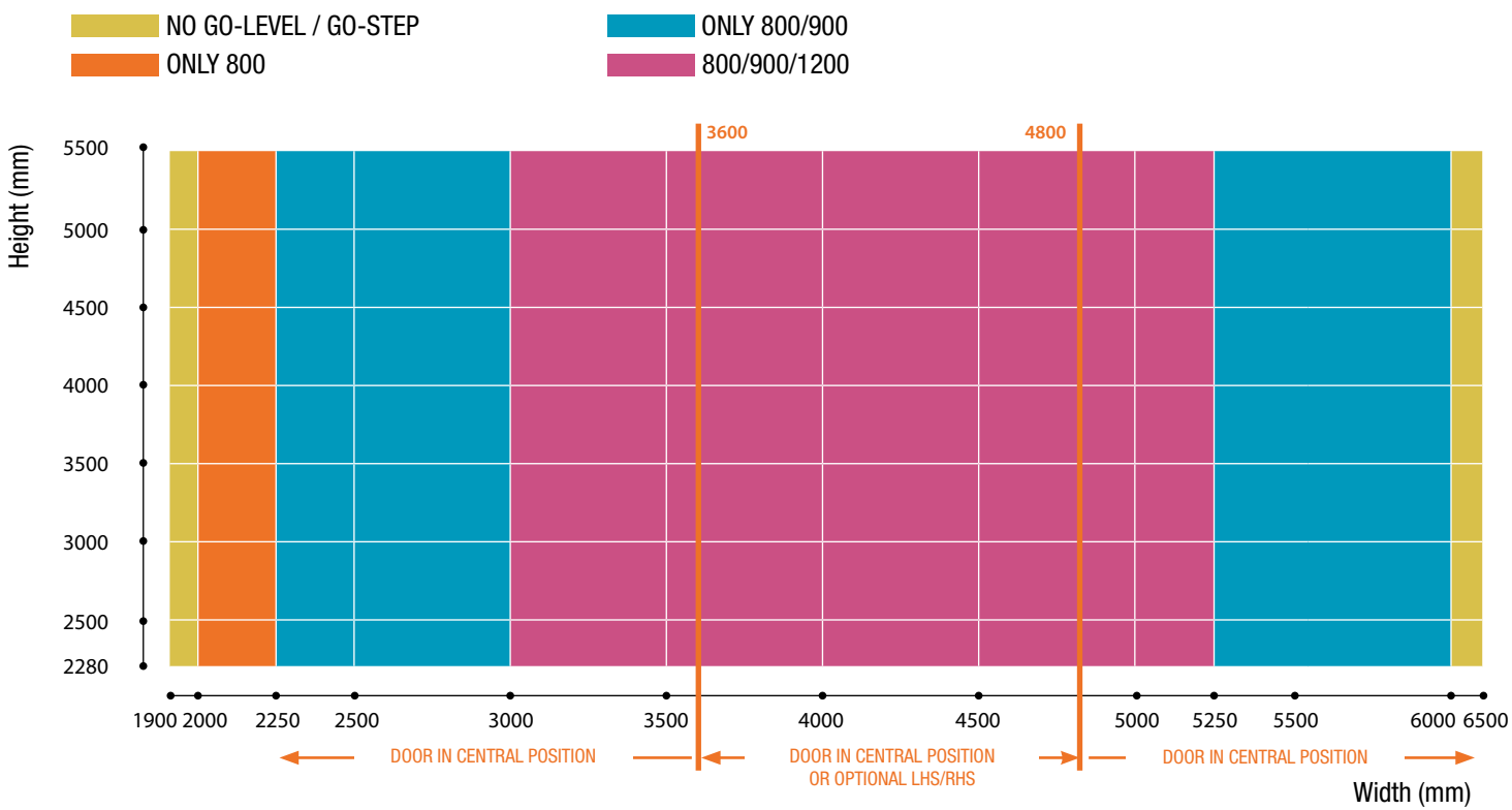
DIAGRAM SHOWING GO-LEVEL / GO-STEP FEASIBILITY ON INDUSTRIAL DOOR
